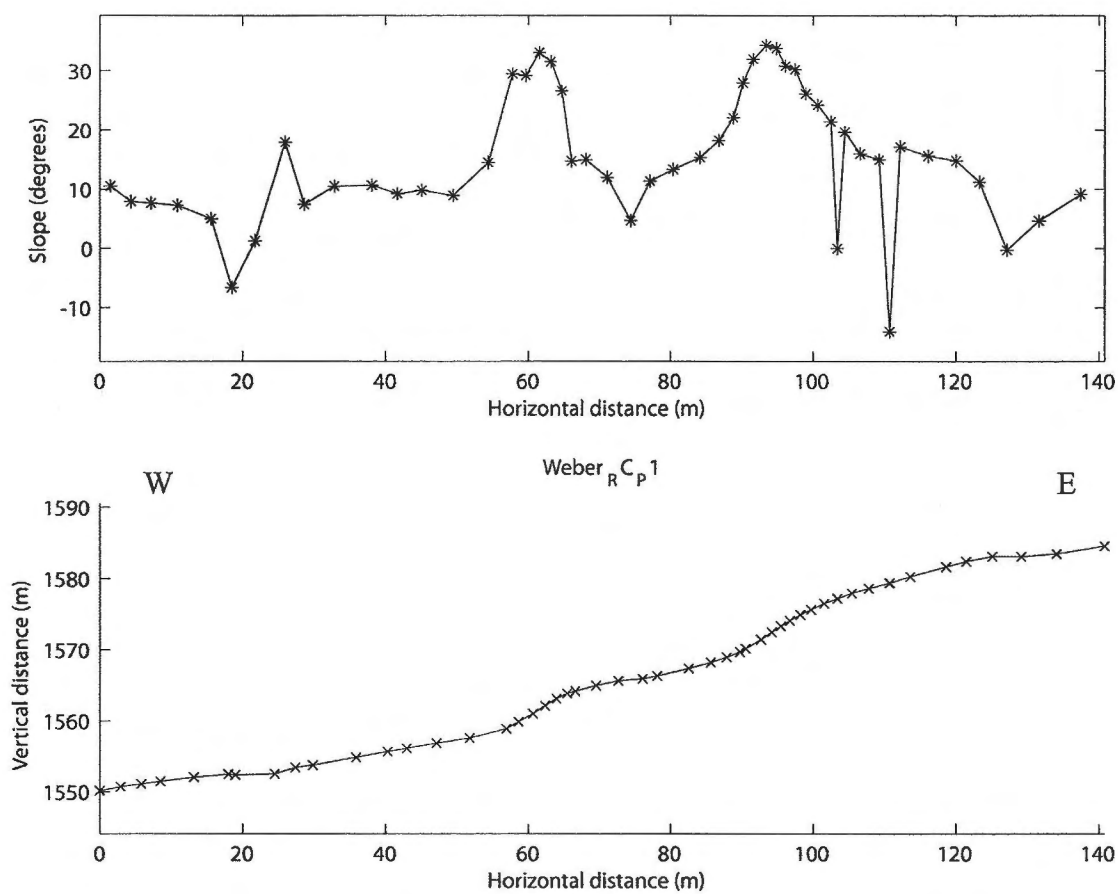
Figure 4. GPS scarp profile collected across the Rice Creek trench site.
