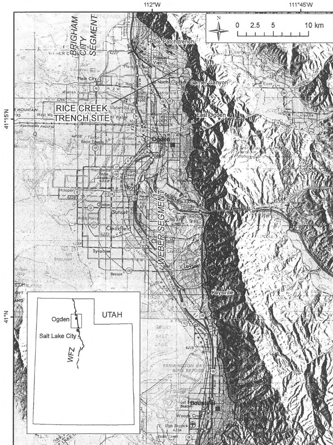
Figure 1. The Weber segment of the Wasatch fault zone, showing existing trench sites (I shapes) and the Rice Creek trench site.
