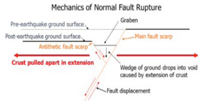
Figure 9. Diagram of typical ground displacements associated with normal faulting such as occurred during the 1983 Borah Peak, Idaho earthquake and is expected during the Salt Lake scenario earthquake. Diagram by T.L. Youd.
