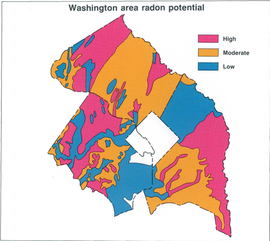
Radon potential, Montgomery and Prince Georges County, Maryland, and Fairfax County, Virginia.
