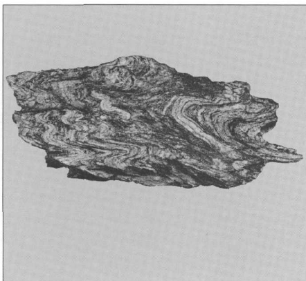
Metamorphic
