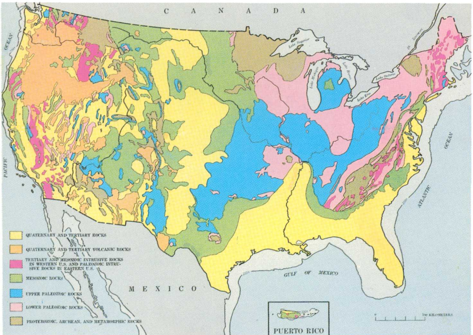
Simplified geologic map of the lower 48 States and Puerto Rico.
