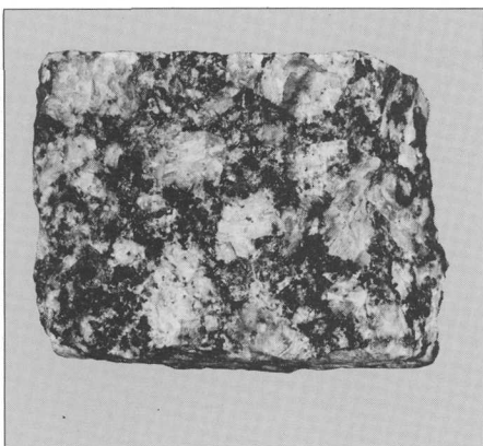
Igneous
