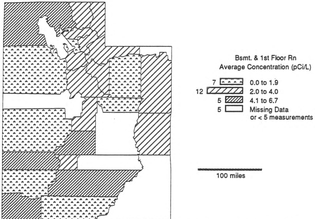
Figure 6. Indoor radon data from the State of Utah Radon Survey (Sprinkel and Solomon, 1990b), for counties with 5 or more measurements. Data are from 1-year alpha-track detector tests conducted during 1987-88. Histograms in map legends show the number of counties in each category. The number of samples in each county (see Table 1) may not be sufficient to statistically characterize the radon levels of the counties, but they do suggest general trends. Unequal category intervals were chosen to provide reference to decision and action levels.
