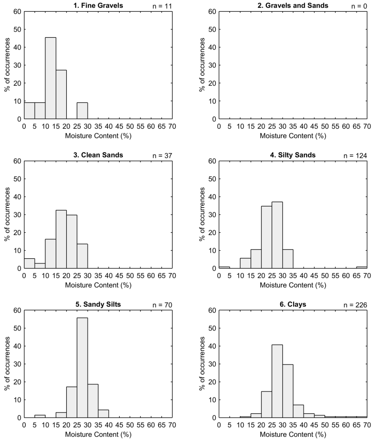
Fig 4.2. Histograms of measured moisture content (in percent) for layers classified as SI = 1 to 6, Utah County geotechnical database.
