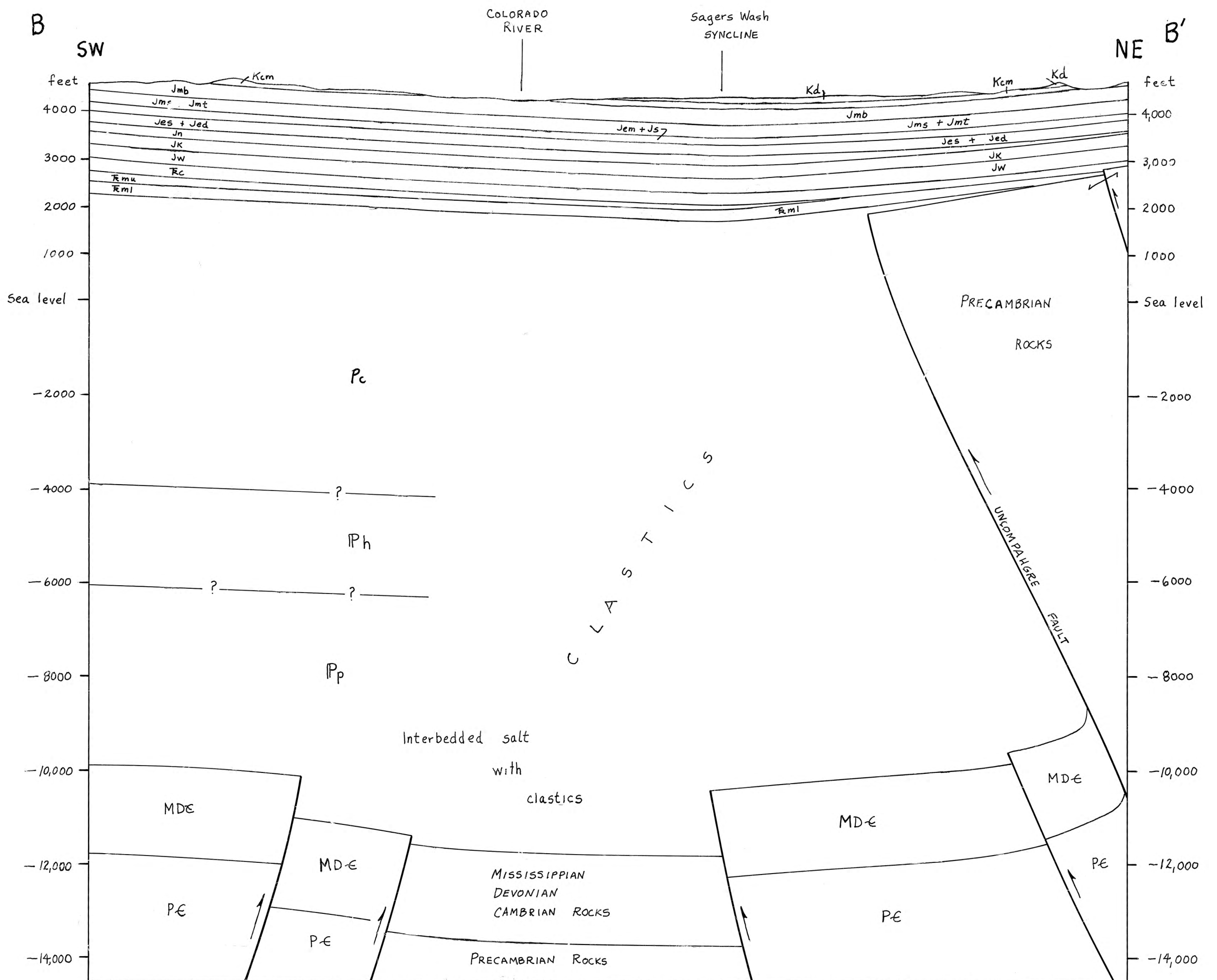
Diagrammatic and conjectural below 3,000 feet, follows model of White and Jacobsen, 1983.
