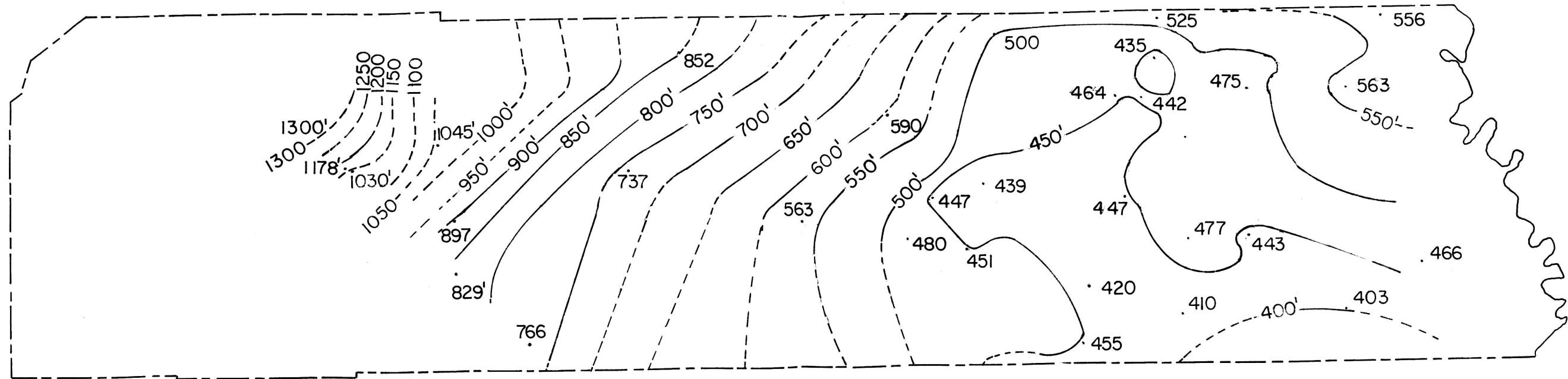
Isopach Map of Moenkopi Formation contour interval 50'
