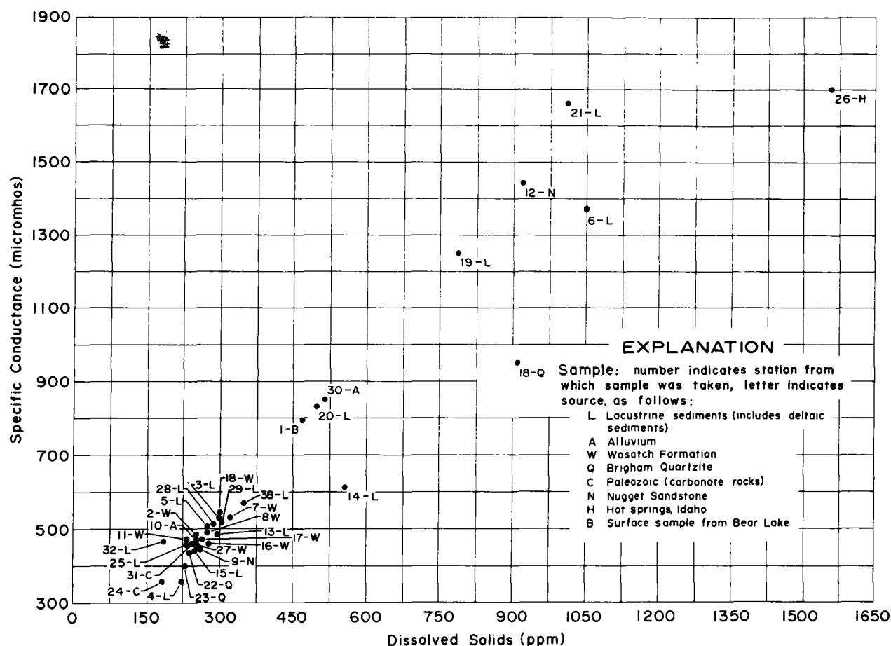
Figure 7. Relation between total dissolved solids and electrical conductivity for groundwaters of the Bear Lake area.
