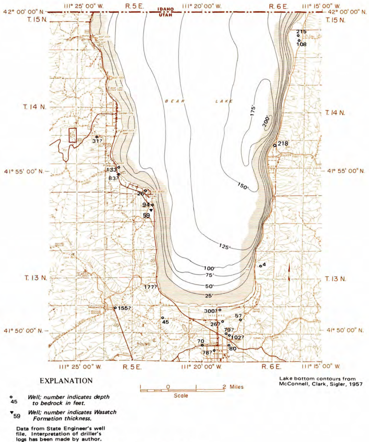
Figure 1. Depths to bedrock and bottom contours of Bear Lake.
