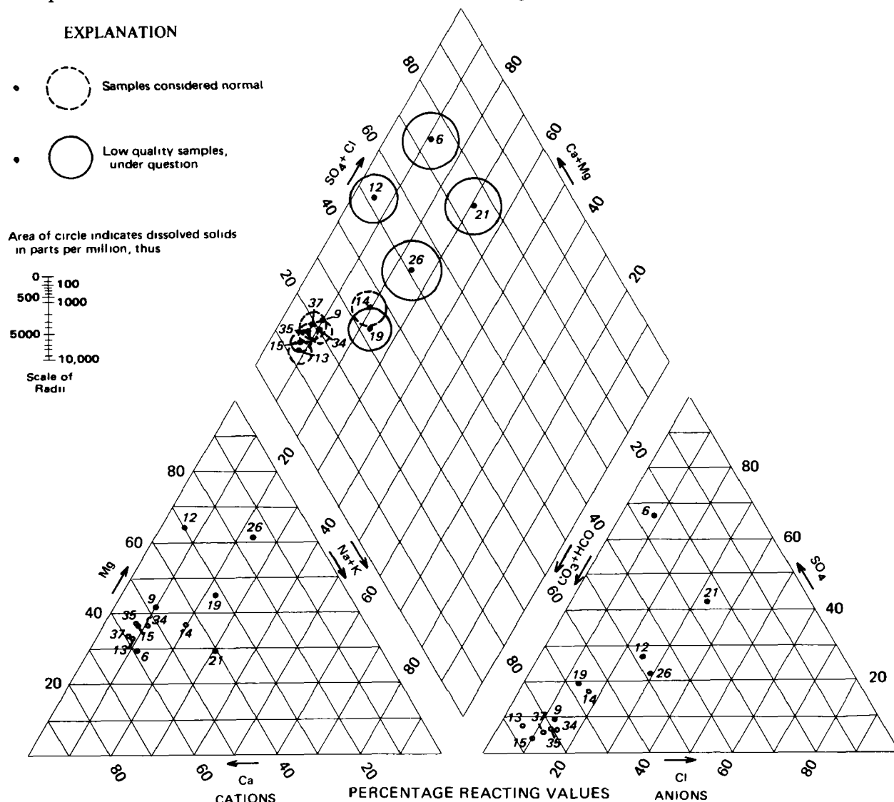
Figure 9. Piper trilinear plot.
