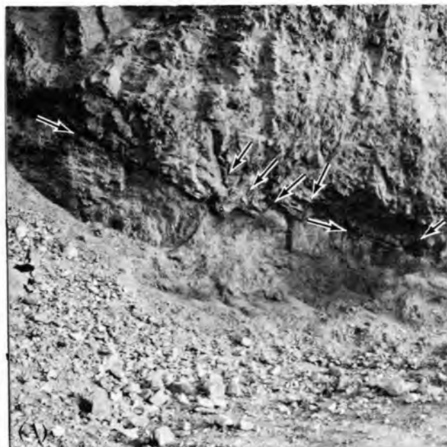
Figure 13. Fault exposures. (A) Faulted Brigham Quartzite exposed in gravel pit, west side of lake (arrows along fault planes show directions of movement). (B) Polished and slickensided Nugget Sandstone exposed at base of hill on east side of lake between North and South Eden canyons.
